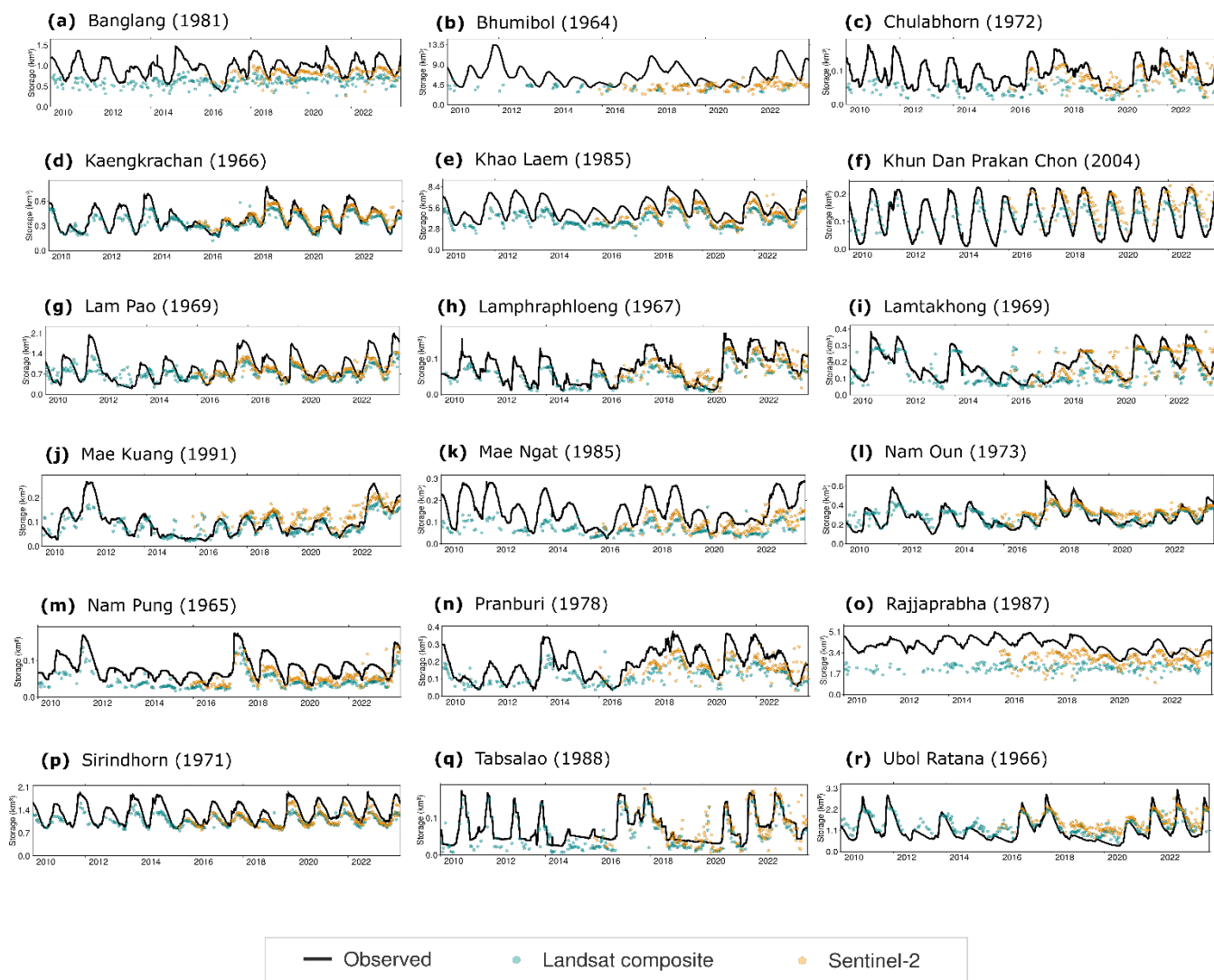
Figure S2: Direct validation of the storage time series against observed storage for eighteen different reservoirs in Thailand. All reservoirs were built before 2000, with the exception of Khun Dan Prakan Chao.
