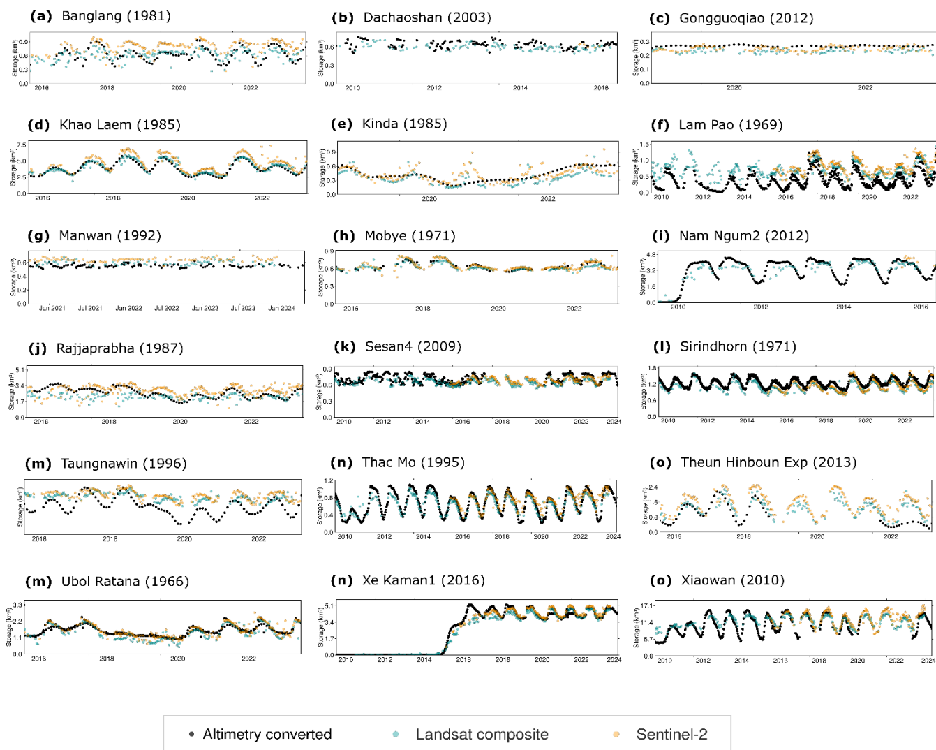
Figure S3: Indirect validation of the storage time-series against altimetry-converted storage for eighteen different reservoirs across Mainland Southeast Asia.
