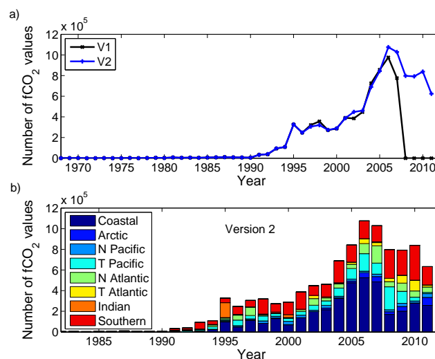
Figure 1. (a) The number of surface water f_{\text{CO}_2} values per year in SOCAT versions 1 and 2 and (b) per region per year in version 2. The SOCAT operationally defined region names are the Coastal Seas, the Arctic Ocean, the North Pacific Ocean, the Tropical Pacific Ocean, the North Atlantic Ocean, the Tropical Atlantic Ocean, the Indian Ocean and the Southern Ocean (Fig. 5, Table 5). These data points originate from data sets with flags of A, B, C or D and have a WOCE flag of 2. The subsequent figures only show f_{\text{CO}_2} values with these characteristics.
